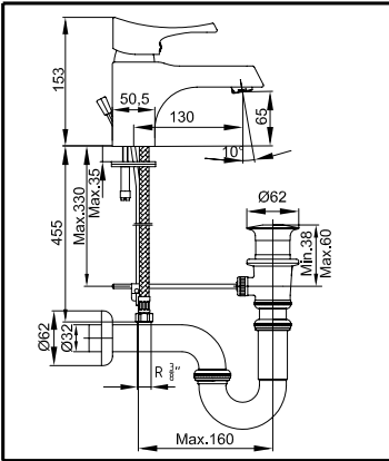
LAVABO BATARYASI KUMANDALI 102108695
